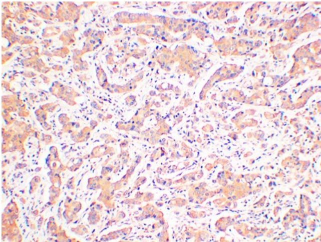
Immunohistochemical analysis of paraffin-embedded Human Breast Carcinoma Tissue using JNK2 Mouse Monoclonal antibody diluted at 1:200.
